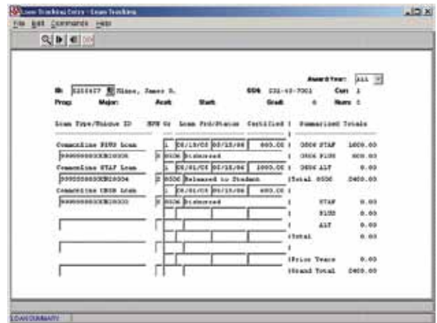
Loan Processing: Loan Tracking Entry Window
